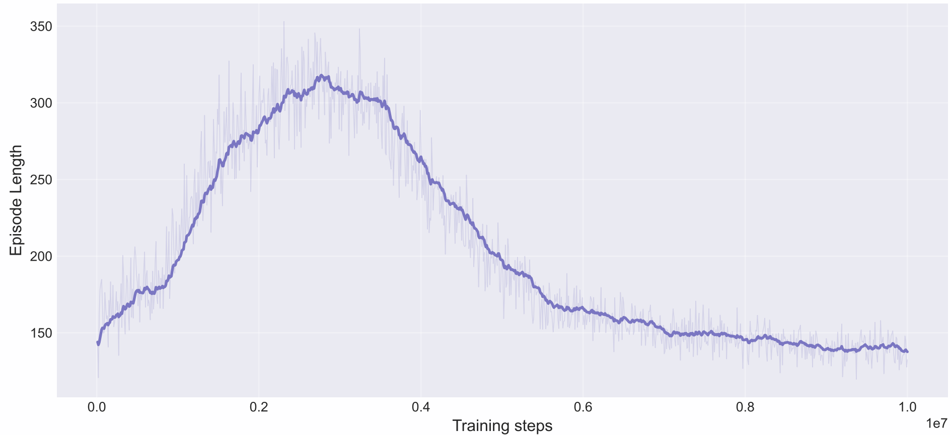
Episode Length
